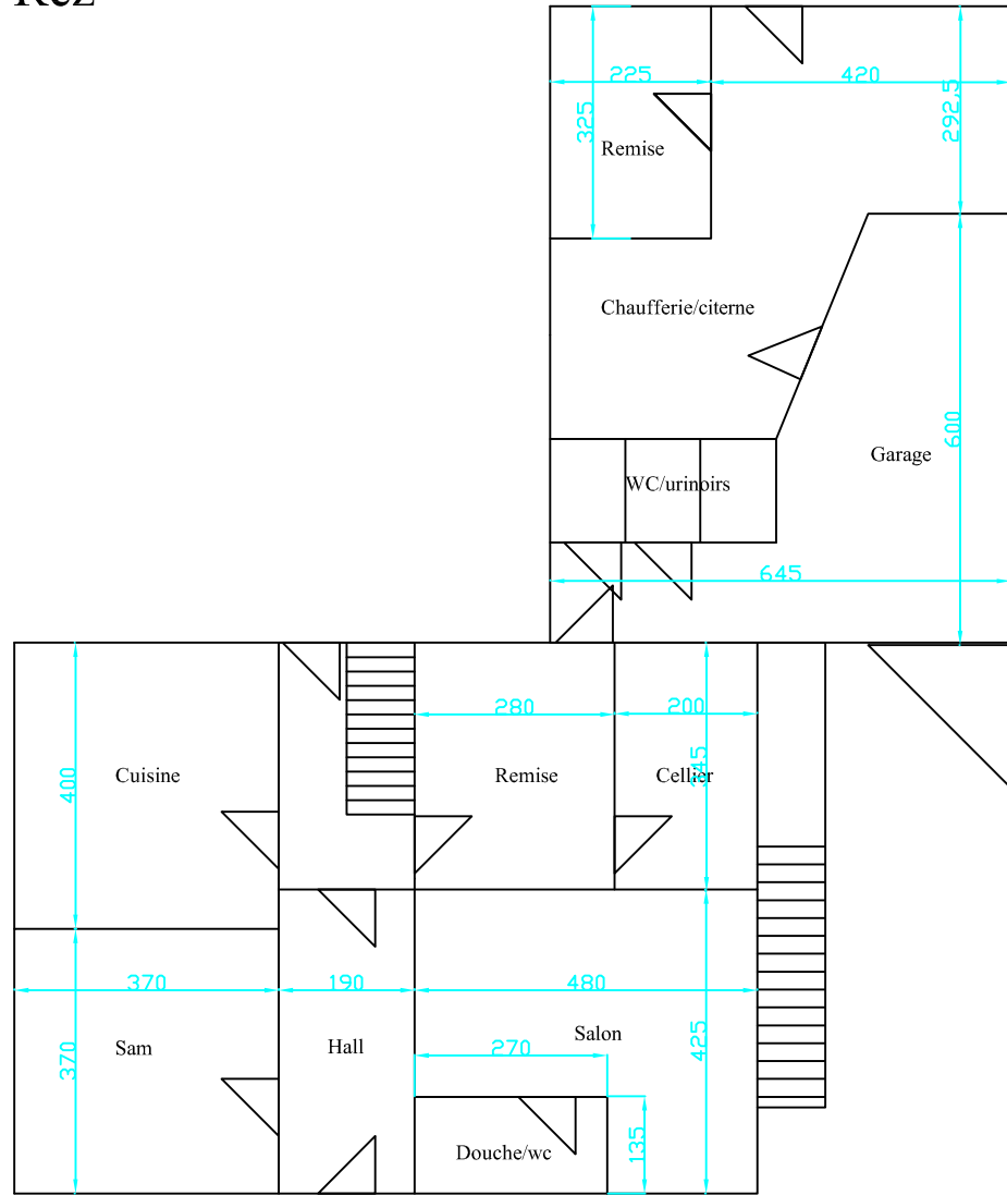
Rez
